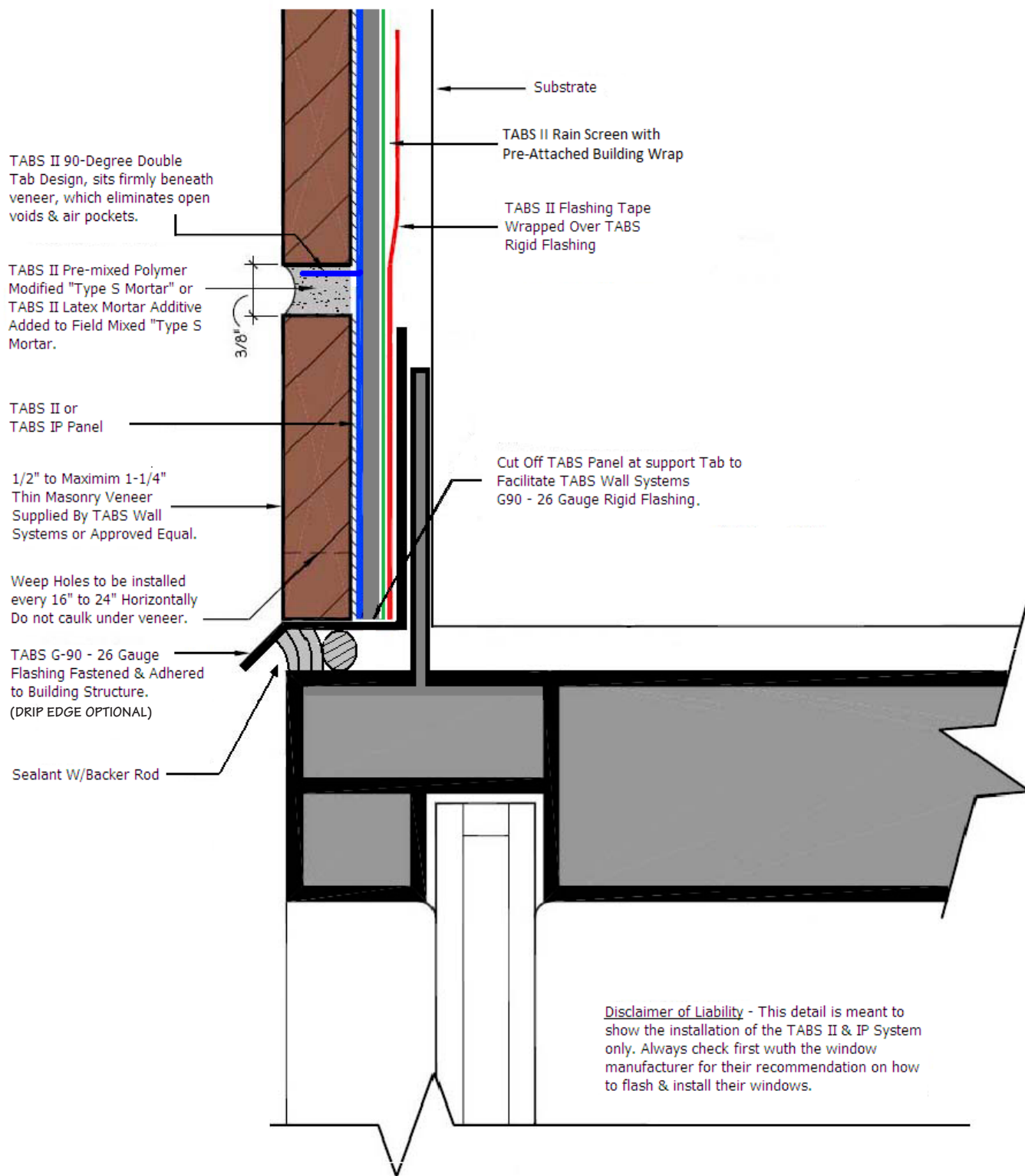
FLANGED WINDOW HEAD SCALE: FULL: / LAST REVISION 10-20-11
