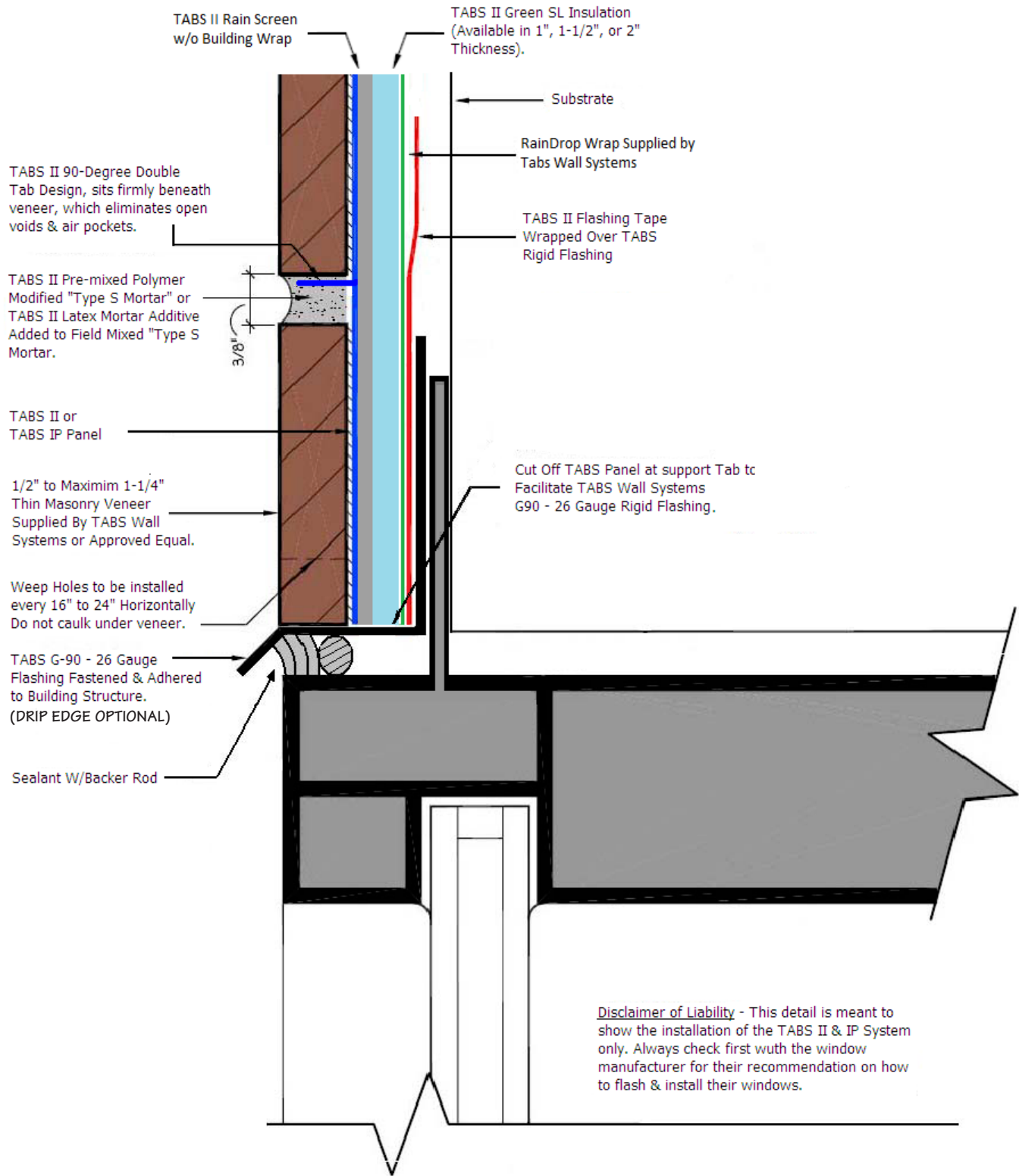
FLANGED WINDOW HEAD SCALE: FULL: / LAST REVISION 10-20-11
