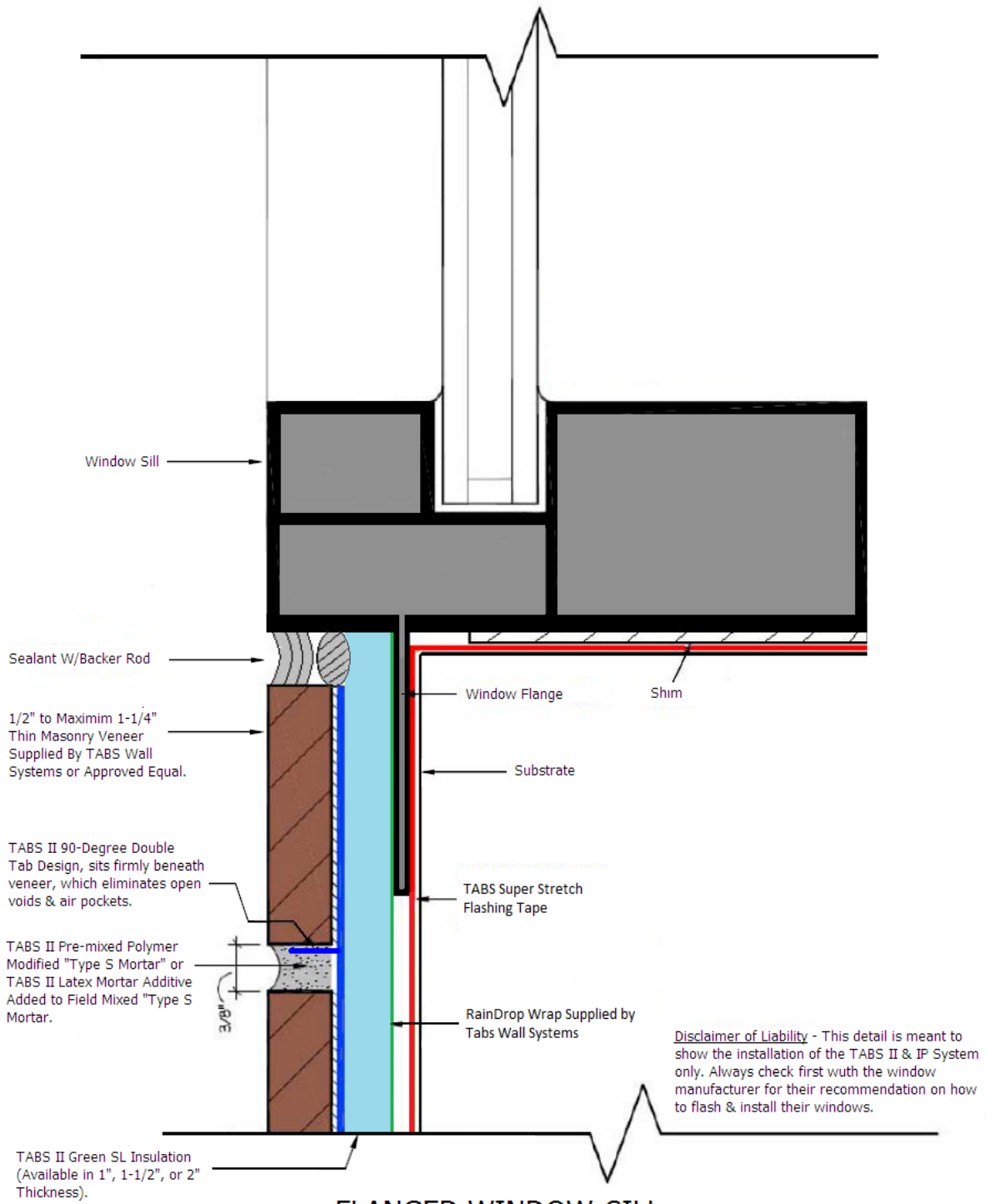
FLANGED WINDOW SILL SCALE: FULL / LAST REVISION: 10-20-11
