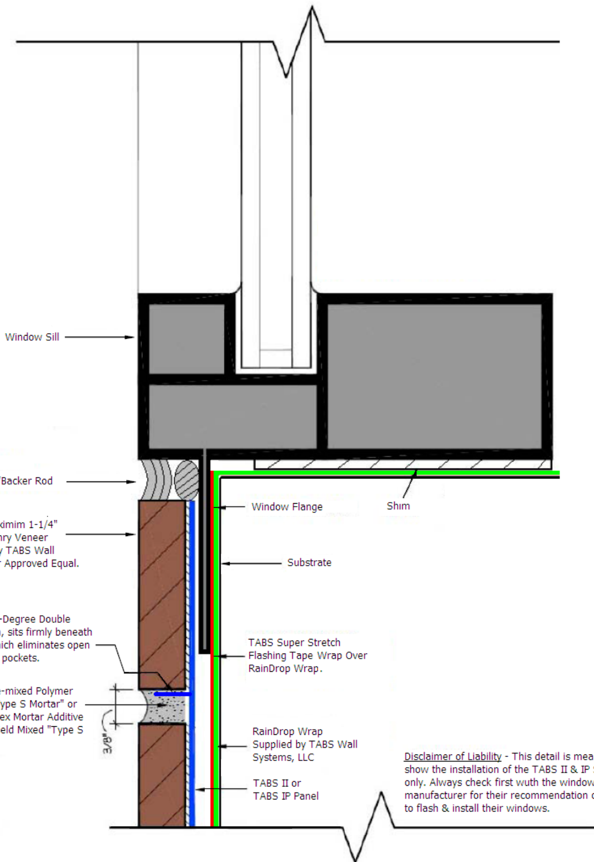
FLANGED WINDOW SILL SCALE: FULL / LAST REVISION: 08-15-09
