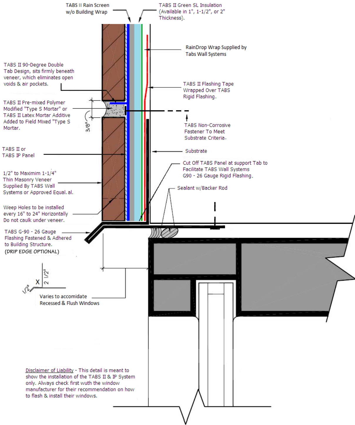
FLUSH & RECESSED WINDOW HEAD SCALE: FULL / LAST REVISION: 10-20-11
