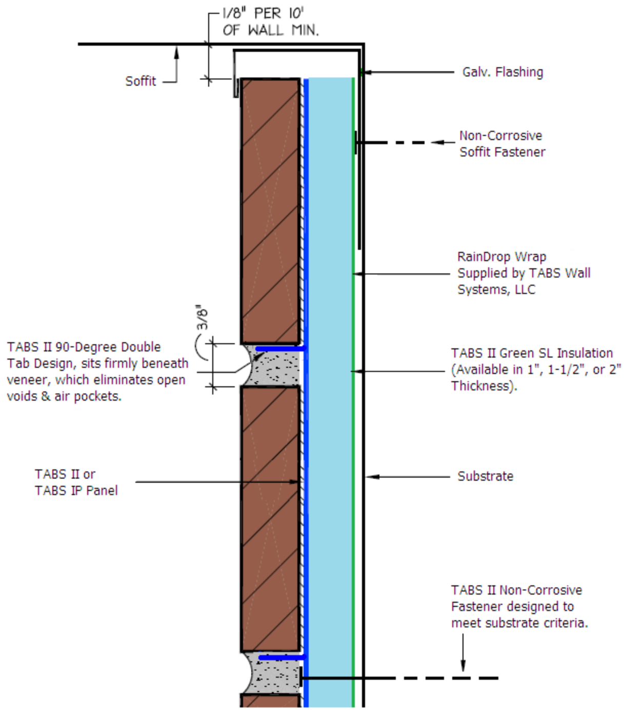
TYPICAL SOFFIT DETAIL SCALE: FULL / LAST REVISION: 10-20-11
