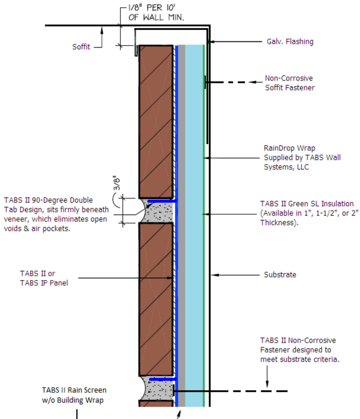
TYPICAL SOFFIT DETAIL SCALE: FULL / LAST REVISION: 10-20-11
