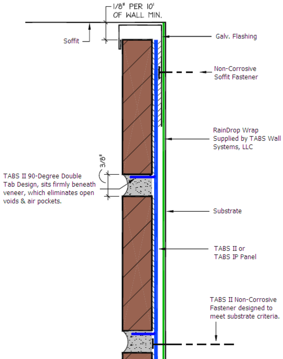
TYPICAL SOFFIT DETAIL SCALE: FULL / LAST REVISION: 08-15-09
